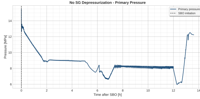
Figure 16: Primary Pressure.
