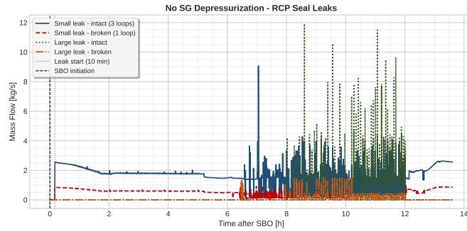
Figure 17: RCP seal leak.
